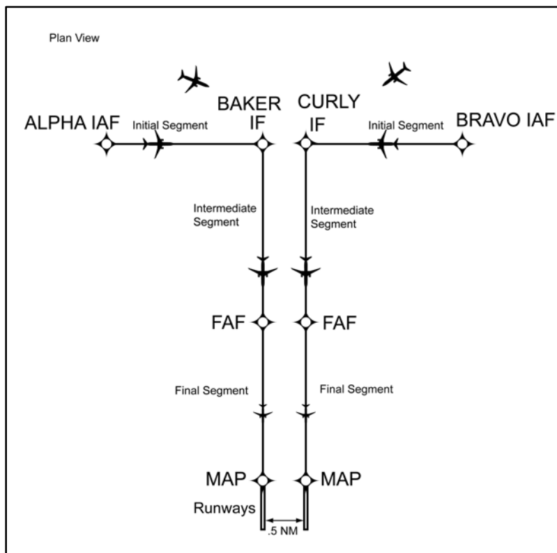
FIG 5-4-4 Modified "T" Approach to Parallel Runways
