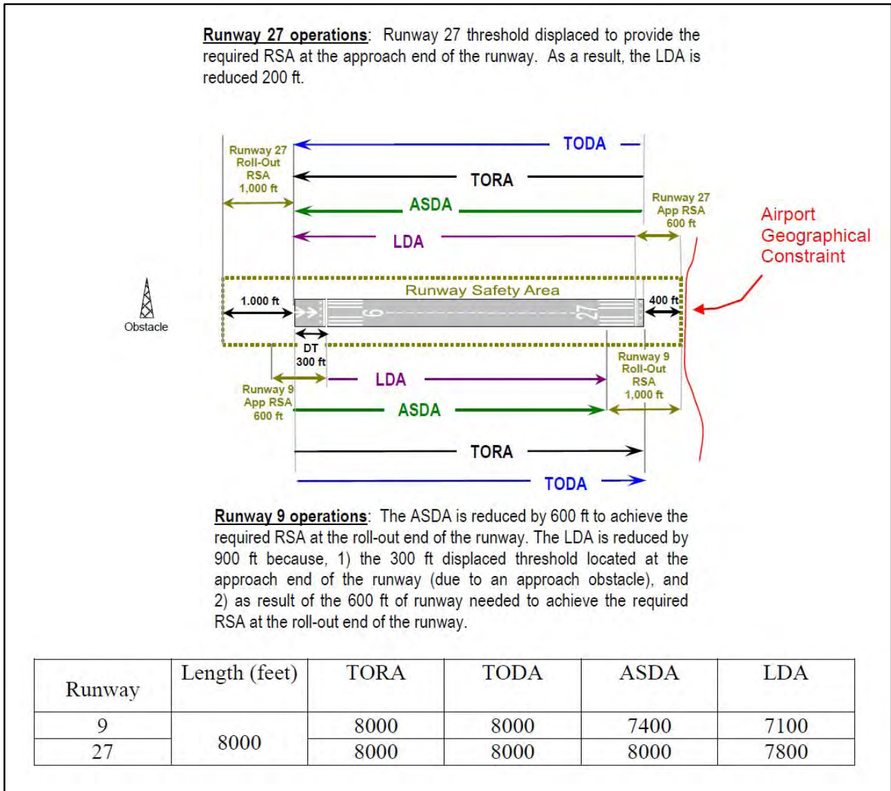
FIG 4-3-5 Effects of a Geographical Constraint on a Runway's Declared Distances
